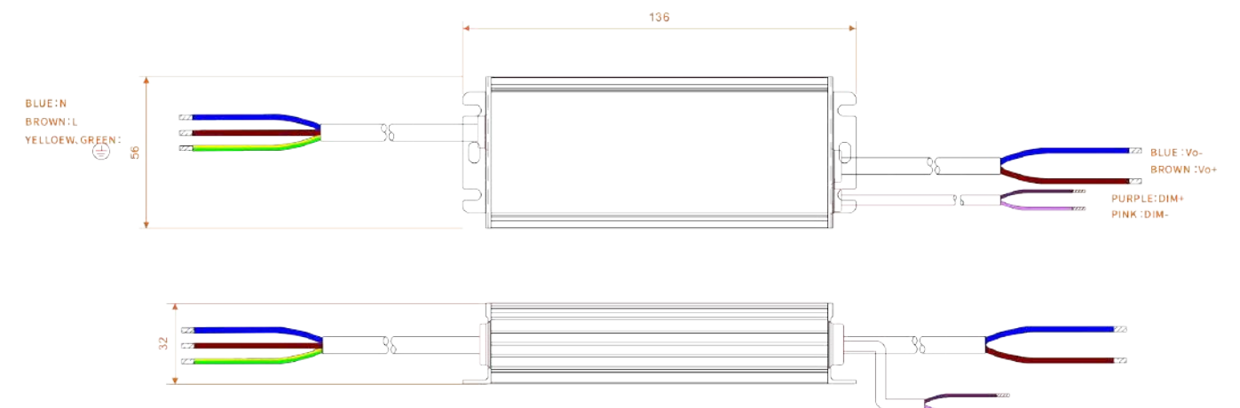
▲ HVS-100W Dimension
